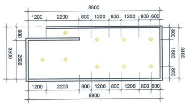
(MEZZANINE FLOOR PLAN) REFLECTED CEILING PLAN SCALE 1:150 MTS
