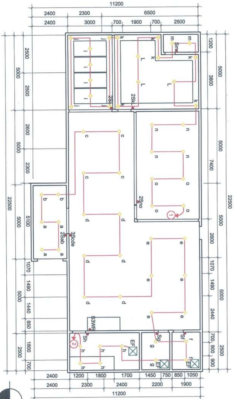
(GROUND FLOOR PLAN) ELECTRICAL LIGHTING LAYOUT SCALE 1:150 MTS
