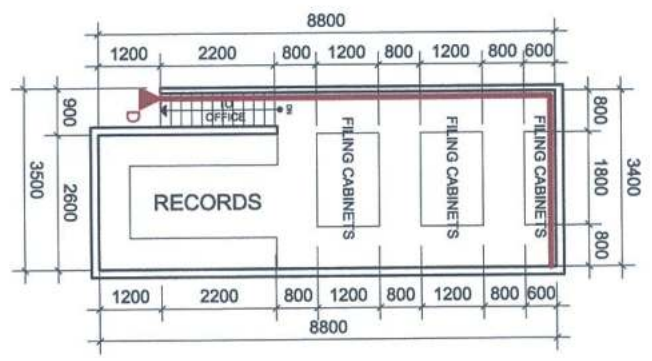
(MEZZANINE FLOOR PLAN) DATA CABLE AND TELEPHONE LAYOUT SCALE 1:150 MTS
