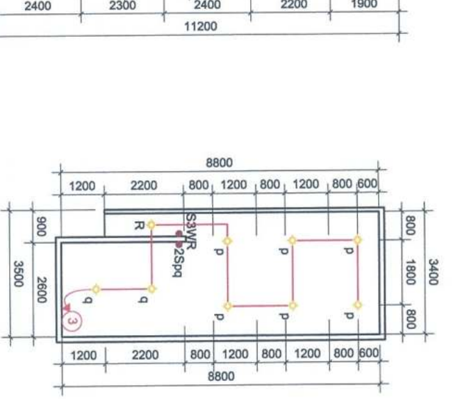
(MEZZANINE FLOOR PLAN) ELECTRICAL LIGHTING LAYOUT SCALE 1:150 MTS
