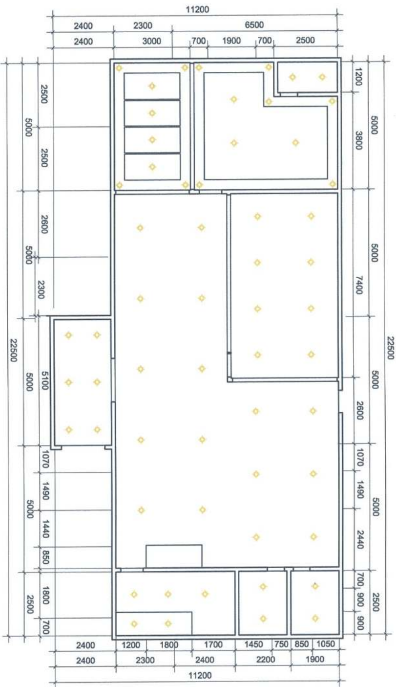
(MEZZANINE FLOOR PLAN) REFLECTED CEILING PLAN SCALE 1:150 MTS
